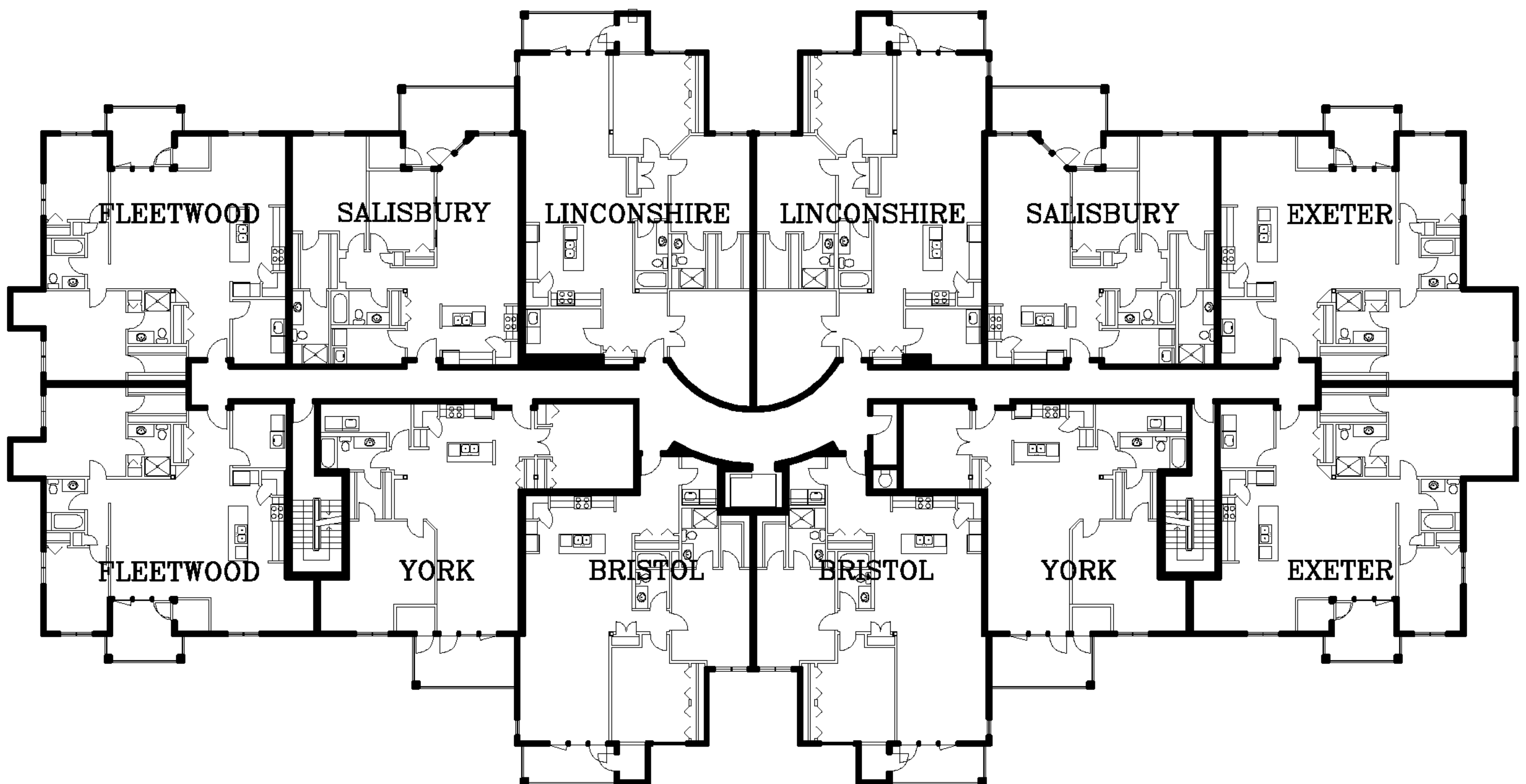
FLOOR PLAN
