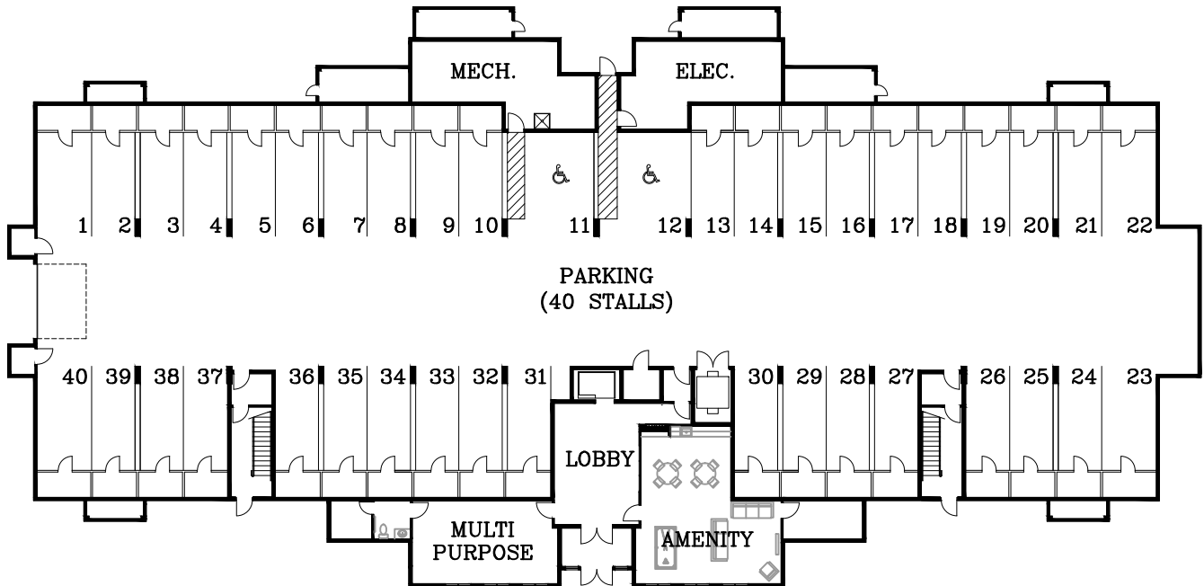
PARKADE PLAN
