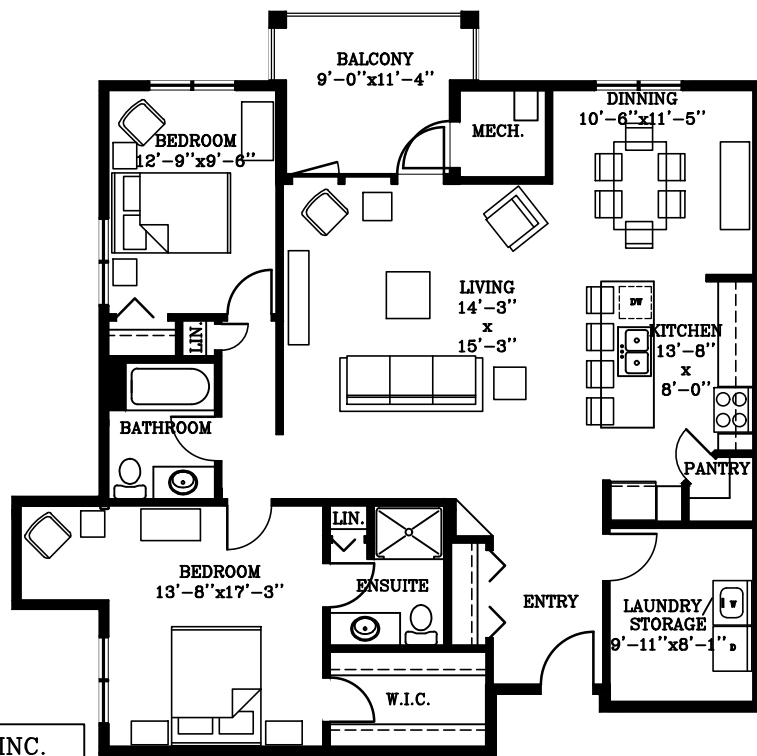
FLEETWOOD SUITE PLAN NORTH 1267 S.F. 204/304/404
