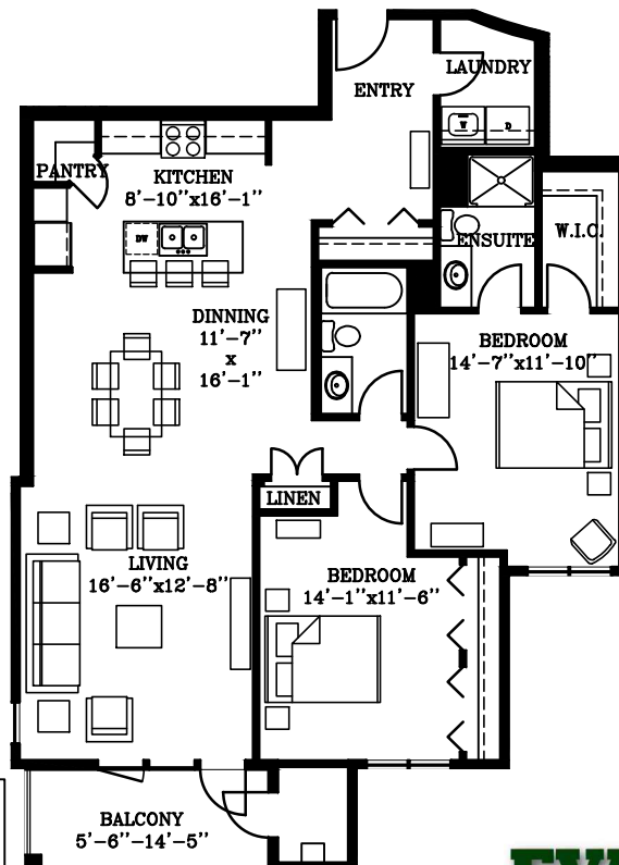
BRISTOL SUITE PLAN WEST 1273 S.F. 201/301/401
