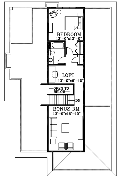
LOFT PLAN OPTION TWO AREA: 720 SQ. FT.
