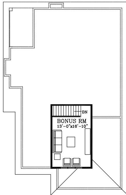
LOFT PLAN OPTION ONE AREA: 301 SQ. FT.
