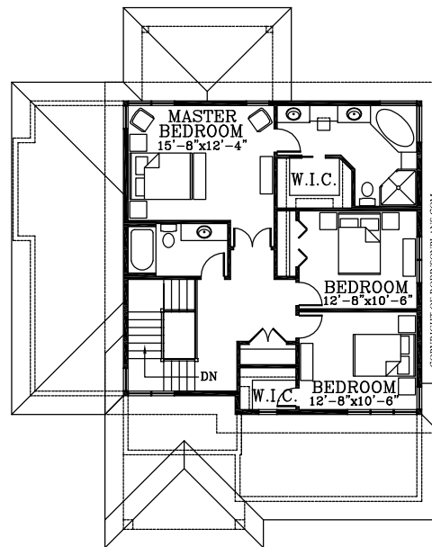
SECOND FLOOR AREA: 1053 SQ. FT.
