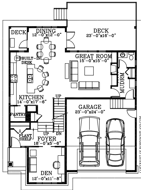
MAIN FLOOR
