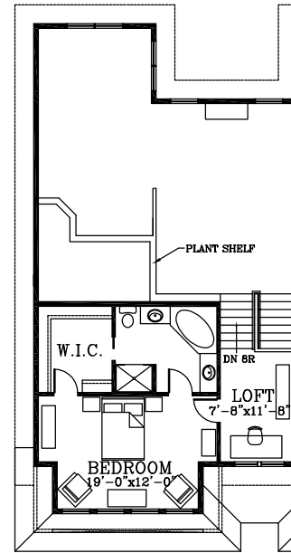
HASTINGS SECOND FLOOR AREA: 570 SQ. FT.
