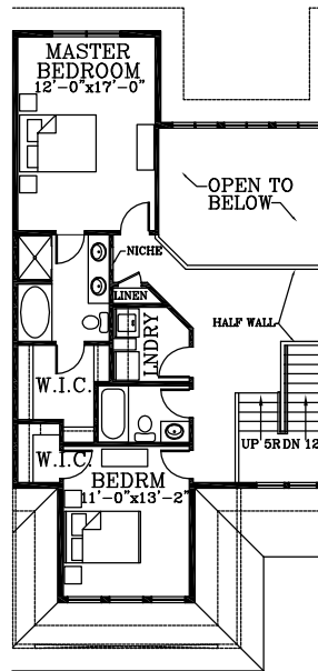
BUXTON SECOND FLOOR OPTION TWO
