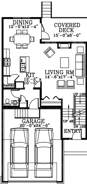
BUXTON MAIN FLOOR
